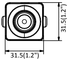
Pinhole Model
