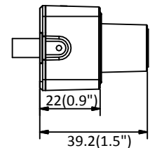
Covert Model
