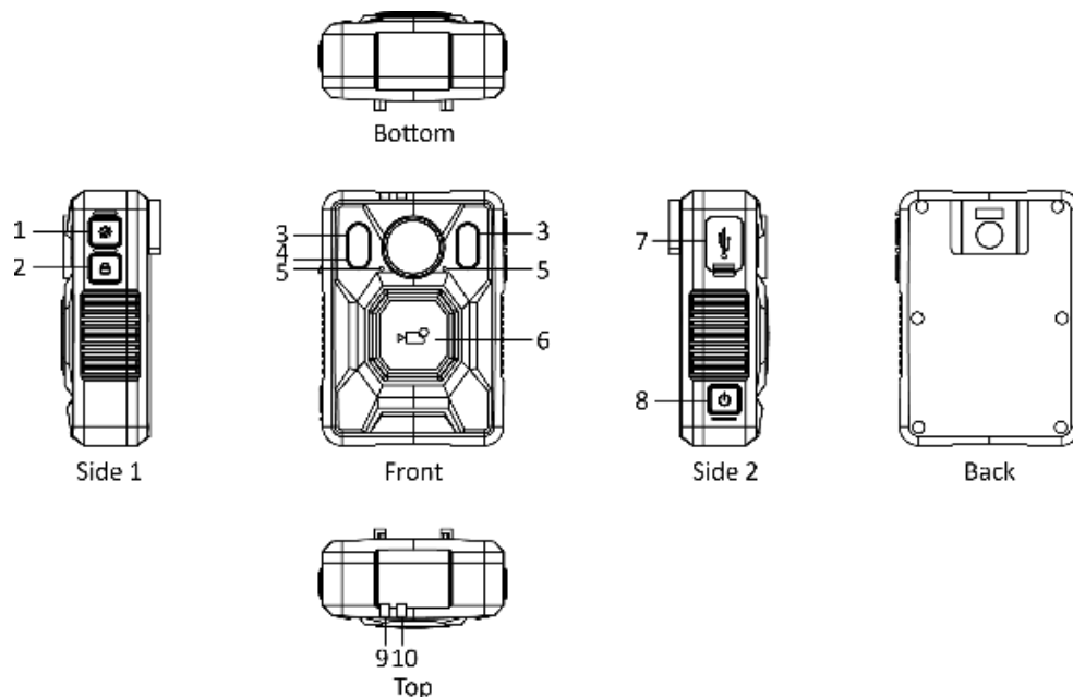
Figure 1, Appearance
