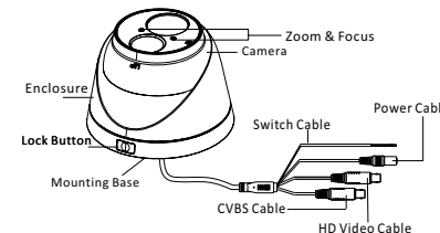
Figure 1-1 Overview of Type I Camera
